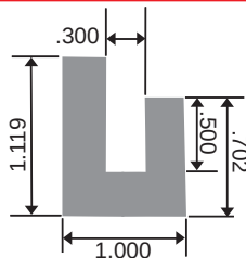
#932-398 SPE-4900-02A1 White Buna
