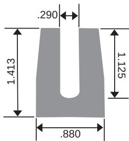
#964-222 SPE-4900-01 Black Buna
