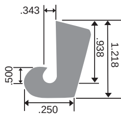
#402-6229 SPE-4900-44 White Buna
