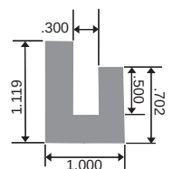
SPE-4900-02 932-398 Tanker Lid Gasket Fabricated
