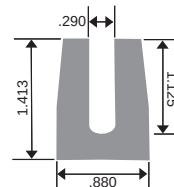
SPE-4900-01 964-222 Universal Fabricated
