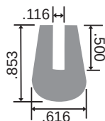
SPE-4900-109 White Buna
