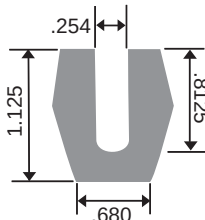
SPE-4900-78 Black Buna SPE-4900-88 White Buna SPE-4900-117 Black EPDM
