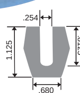
SPE-4900-23K 41186-B Double Flanged Fabricated
