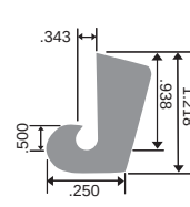
SPE-4900-44 402-6229 Single Flanged Molded
